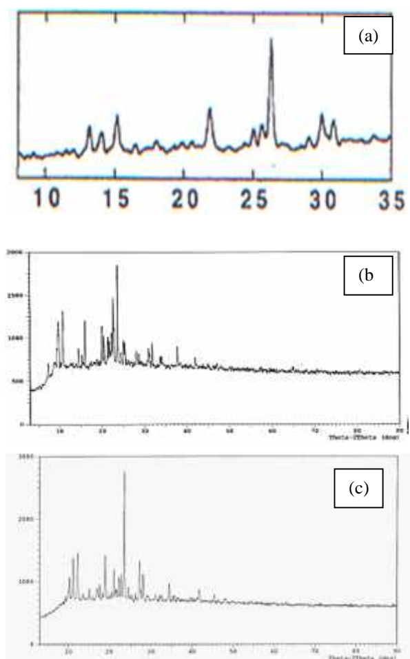
Gambar 4. Pola Difraksi Sinar-X Kompleks (a) [\text{Fe}(\text{fen})(\text{NCS})_2] (Tscuhiya dkk, 2000), (b) Kompleks [\text{Fe}(\text{fen})(\text{NCS})_2] (Joris, 2011) dan (c) Kompleks \{[\text{Fe}(\text{fen})(\text{NCS})_2]_2\text{oks}\} Hasil Sintesis.
